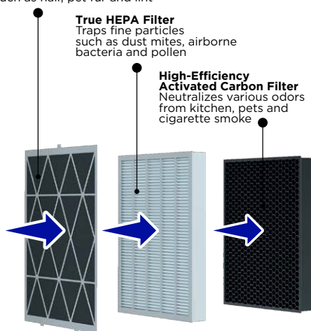
3-Layered Filter System
